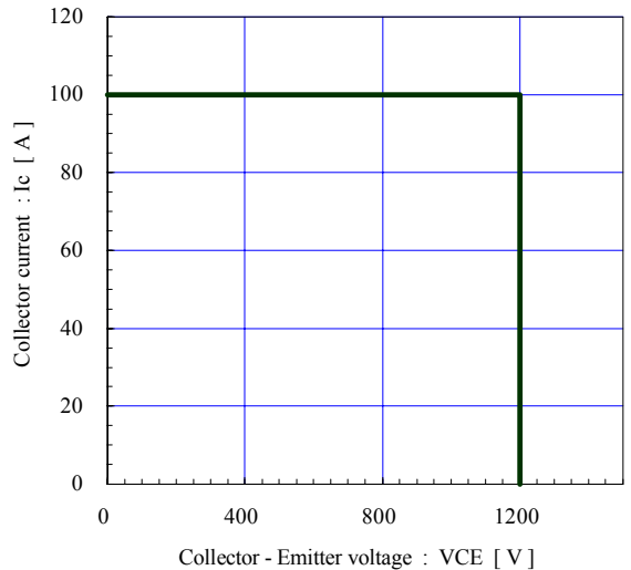
[ Inverter ] Reverse bias safe operating area (max.) +V_{GE}=15V, -V_{GE} \le 15V, R_g \ge 33\Omega, T_j \le 125^\circ C
