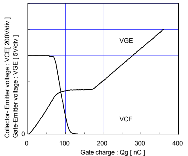
Dynamic Gate charge (typ.) Vcc=600V, Ic=75A, Tj=25°C
