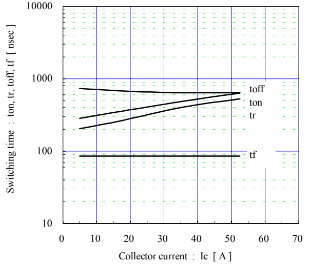
[ Inverter ]
