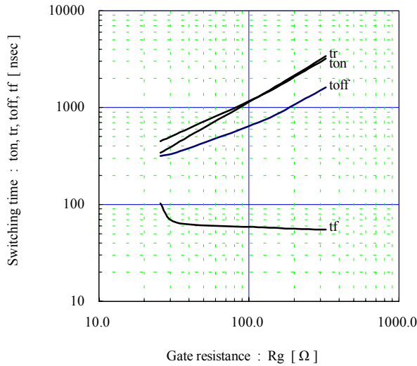
[ Inverter ]
