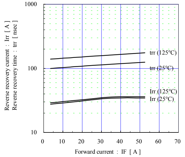
[ Inverter ] Reverse recovery characteristics (typ.) Vcc=600V, VGE=±15V, Rg=33Ω
