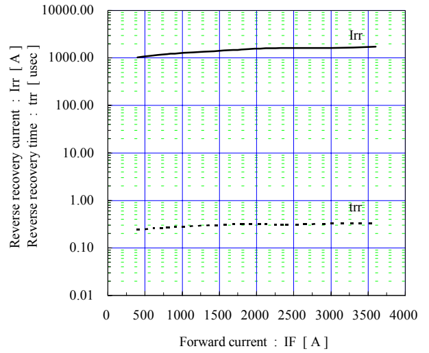
Reverse recovery characteristics (typ.) Vcc=600V, VGE=±15V, Rgon=0.9Ω, Tj=125°C
